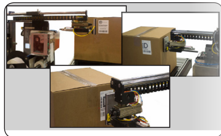
Model 252 3-panel label printer applicator with choice of proven OEM print engine (SATO, Zebra, or Datamax.)
